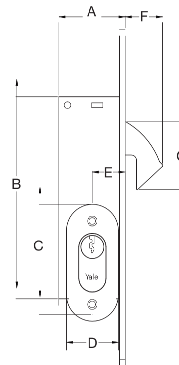
MEDIDAS EN mm / MEASURES IN mm
